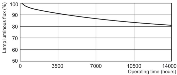
Lumen Maintenance Diagram - MASTER PL-S 11W/840/2P 1CT/10
